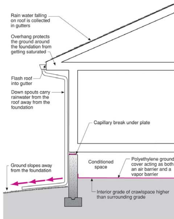
Figure 1 Groundwater Control with Crawlspaces
