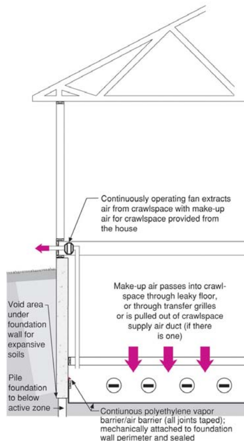
Figure 4 Combined Controlled Ventilation, Soil Gas and Crawlspace Ventilation System
