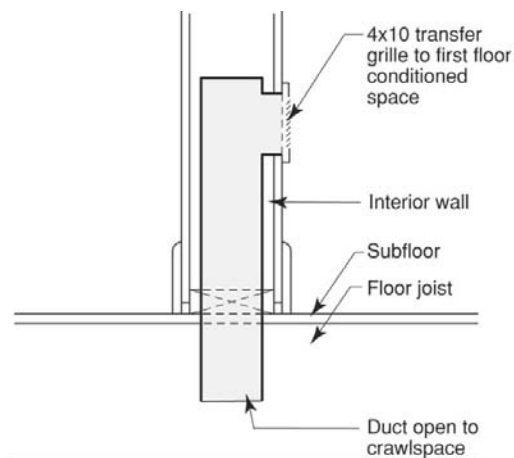
Figure 5 Transfer Grille to Crawlspace
