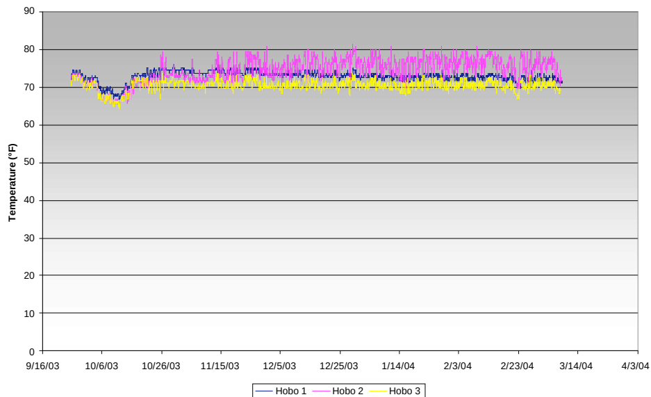
Graph 10: Albuquerque House Crawlspace Temperature
