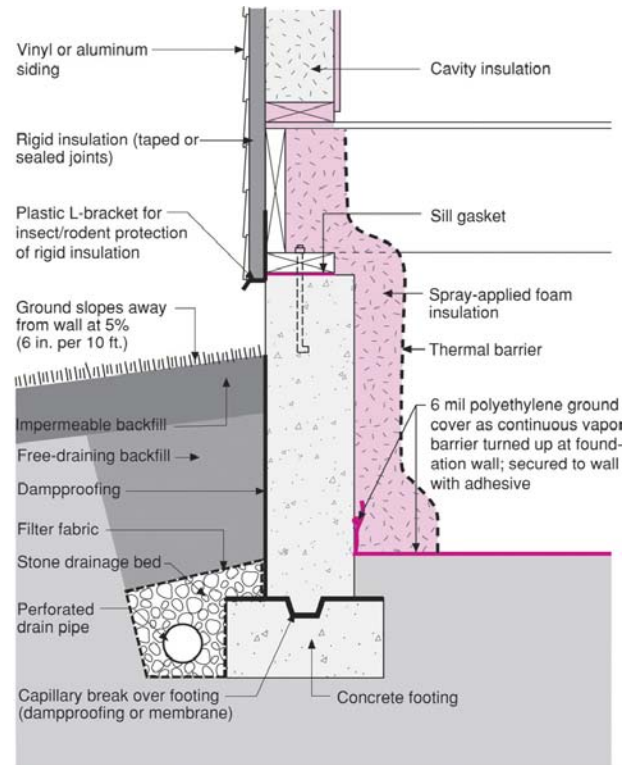
Figure 11 Internally Insulated Concrete Crawl Space with Spray Foam
