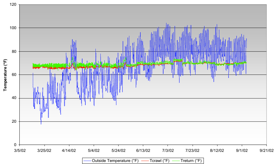
Graph 1: Cleveland House Indoor, Outdoor, and Crawl Space Temperatures
