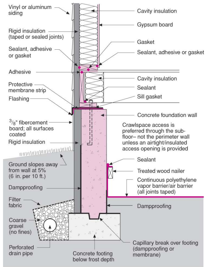
Figure 10 Externally Insulated Concrete Crawl Space with Vinyl or Aluminum Siding Above
