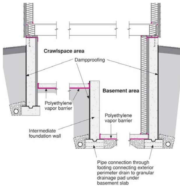
Figure 6 Connecting Crawlspace and Basement
